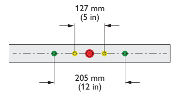
Mounting bracket dimensions for pre-drilling
