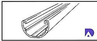
CTGB-AL6.0: Channel base T6 aluminium mill finish. 6 metre length. 3.75kg per length
