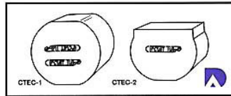
CTEC-1: Rounded end cap. PVC. Black, Grey, White. CTEC-2: Flat end cap. PVC. Black, Grey, White.
