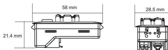
Movement detector (PIR), remote control receiver (IR) and photocell (CL) dimensions
