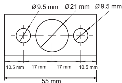
Movement detector (PIR), remote control receiver (IR) and photocell (CL) dimensions
