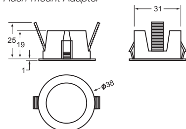
Flush-mount Adapter
