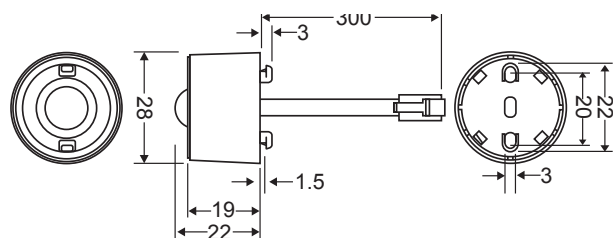
Flush-mount Adapter
