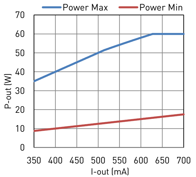
Output Power
