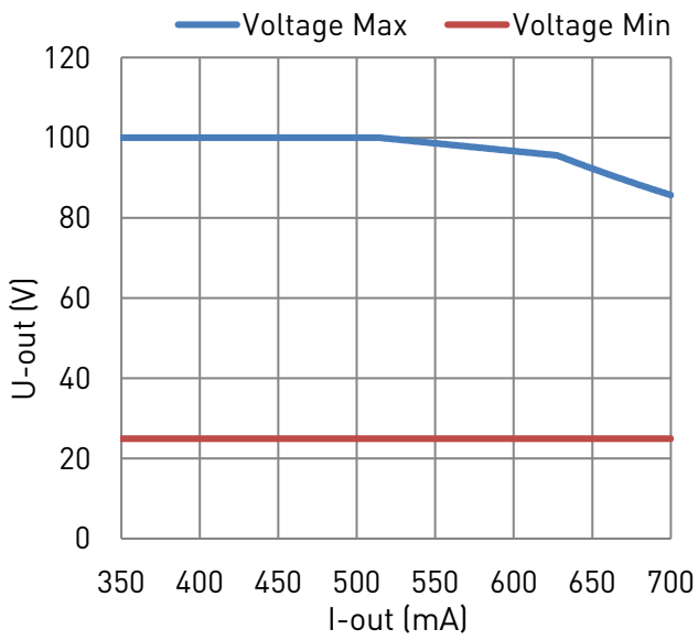
Output Voltage
