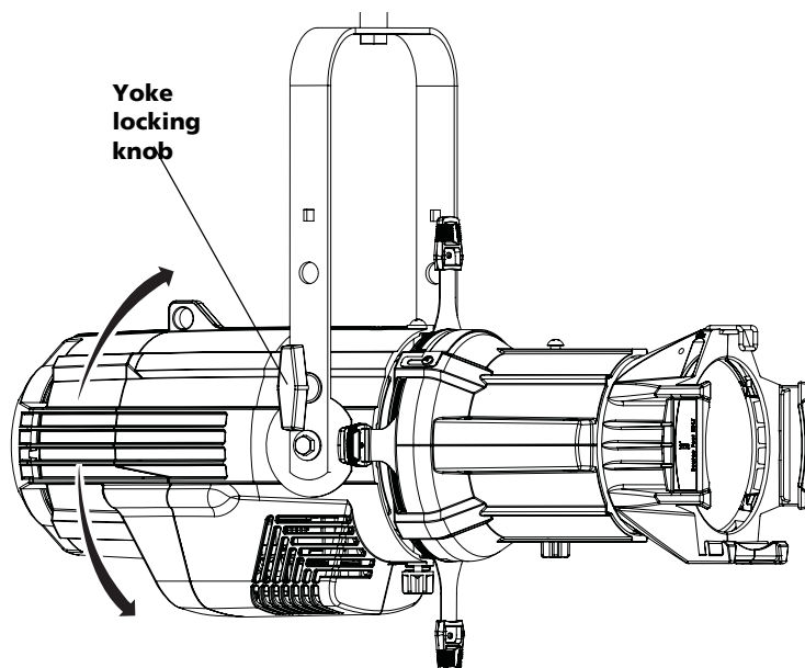
Figure-1.3 Tilting the Fixture on the Yoke.
