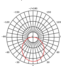
Candle power distribution
