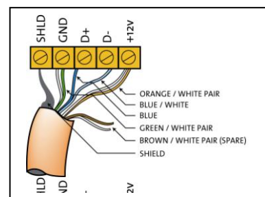
Serial Cable Permanent Connections
