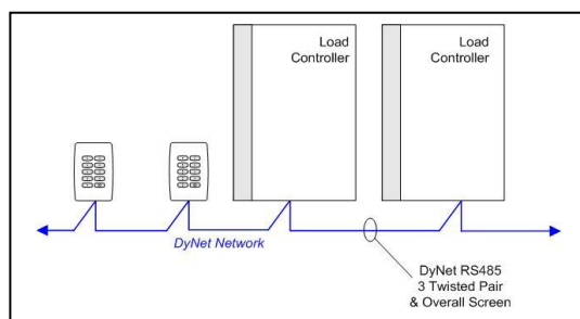
Connect Data Cable in a 'Daisy Chain'
