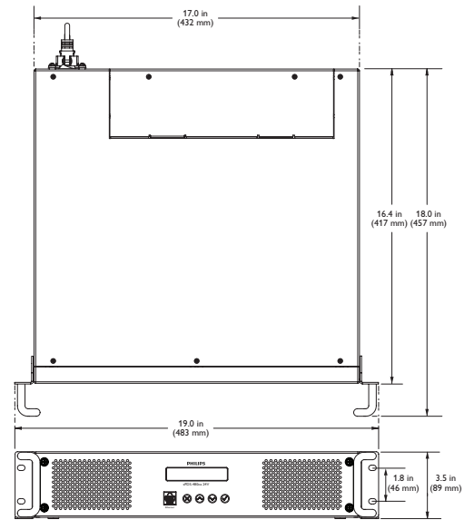
Dimensions: Rack Mount Configuration
