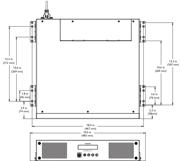
Dimensions: Rack Mount Configuration
