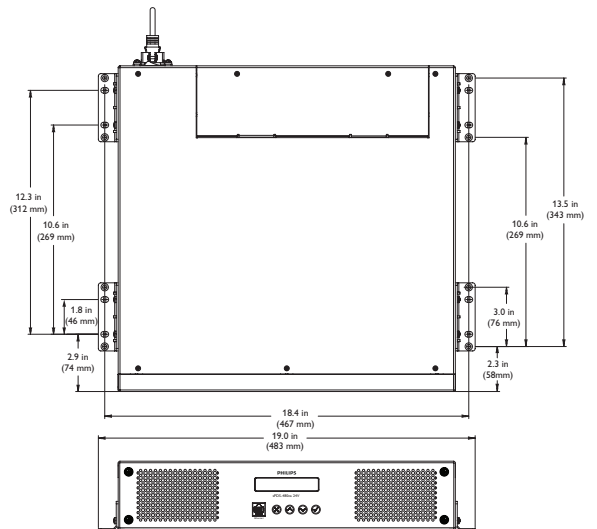
Dimensions: Surface Mount Configuration
