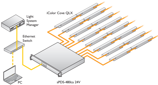
Typical iColor Cove QLX Installation
