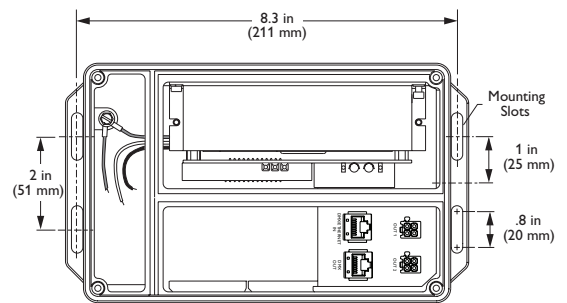
Mounting Dimensions
